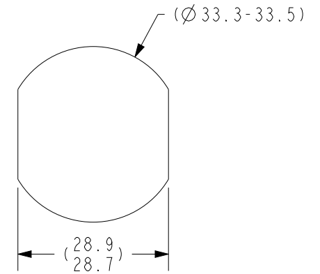
TYPICAL PANEL CUTOUT
