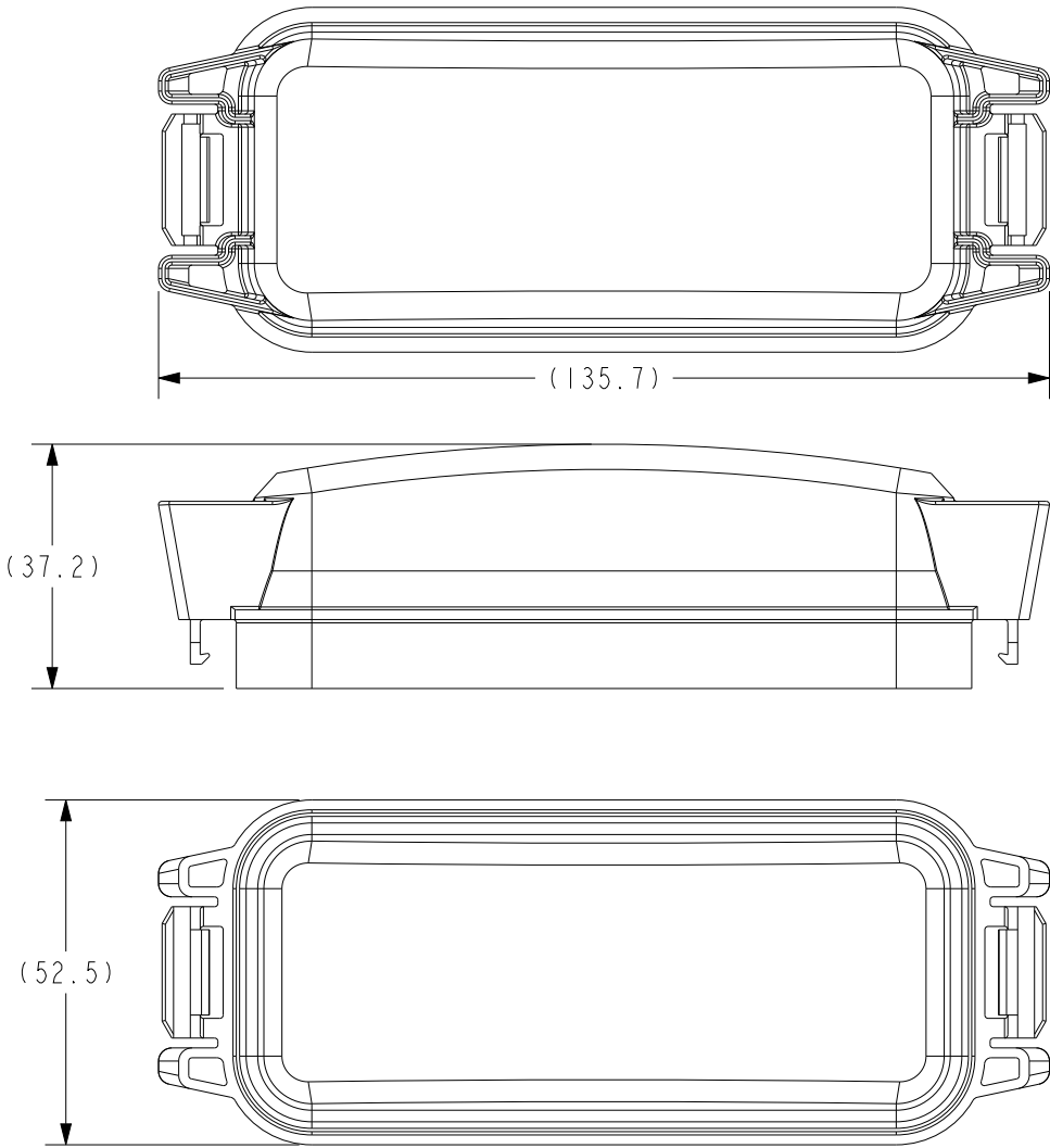
PDM-TCP COVER, PLAIN
