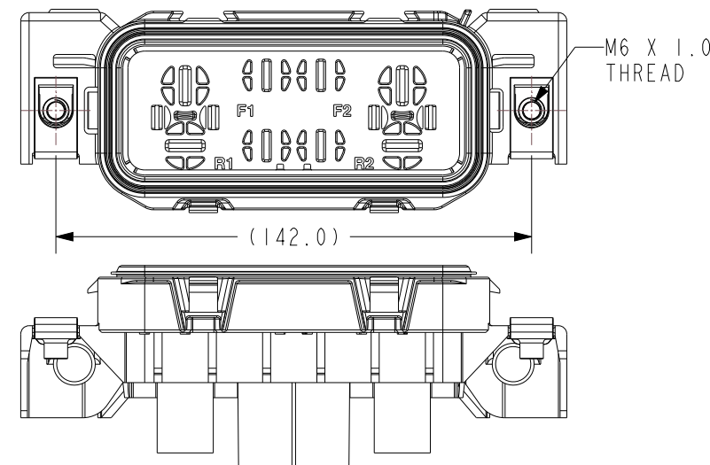
SC42-2033C-A001 HOUSING AND SEAL - PDM-R - MAXI ISO RELAY AND MAXI FUSE - TM CLPS
