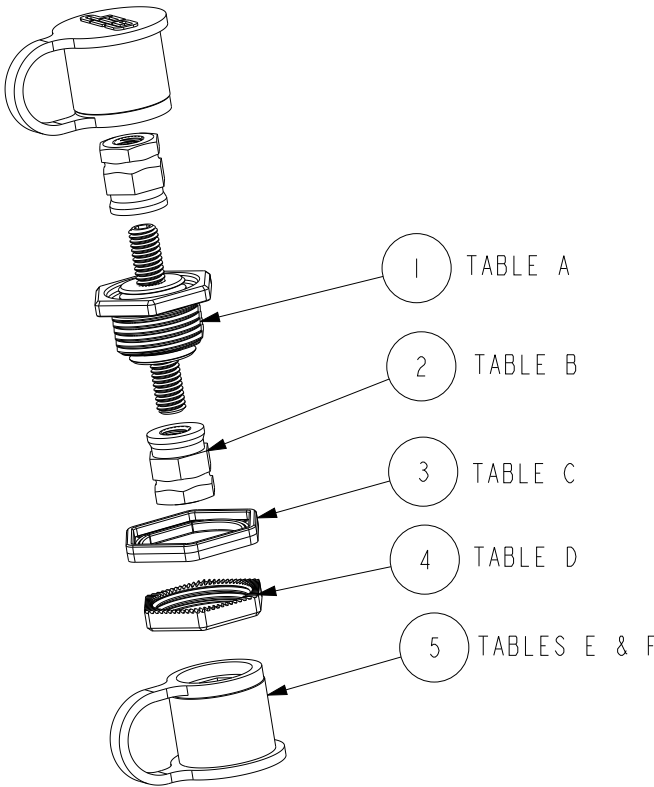
EXAMPLE CONFIGURATION EXPLODE VIEW
