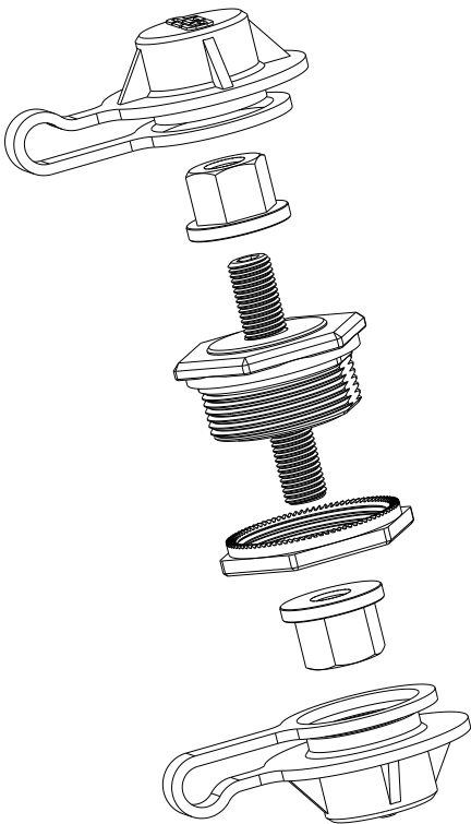
EXPLODE VIEW
