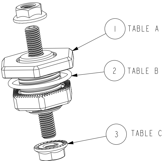
EXAMPLE CONFIGURATION EXPLODE VIEW
