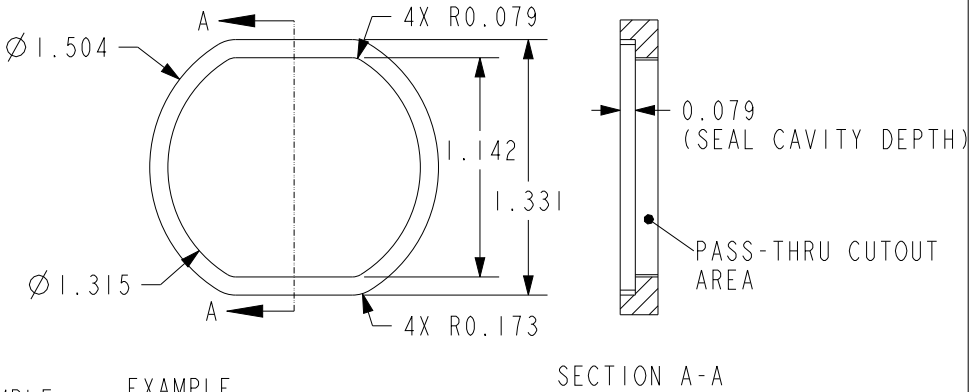
C14-1003 SEAL CAVITY GEOMETRY
