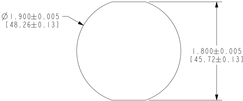
TYPICAL PANEL CUTOUT STYLE C
