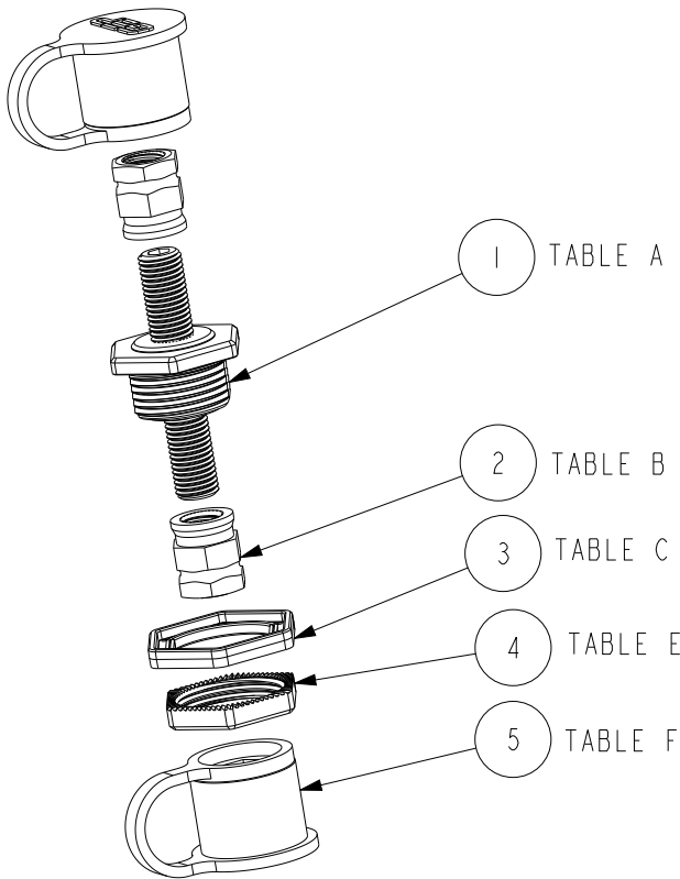
EXAMPLE CONFIGURATION EXPLODE VIEW
