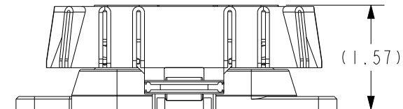
COVER CLOSED
