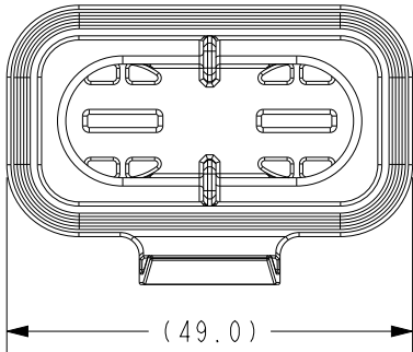
SC42-2007A-B001 HOUSING AND SEAL - PDM - FRH MAXI - 32V
