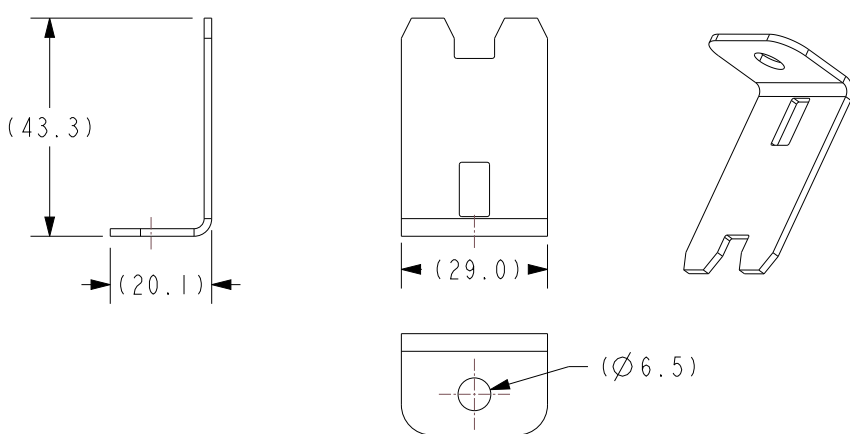
FRH-A12-MB-C2 BRACKET - PDM, FRH, 90° BENT, STAINLESS 304
