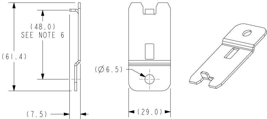
FRH-A12-MB-A1 BRACKET - PDM,FRH,FLAT WITH ANTI-ROTATION, ZINC STEEL
