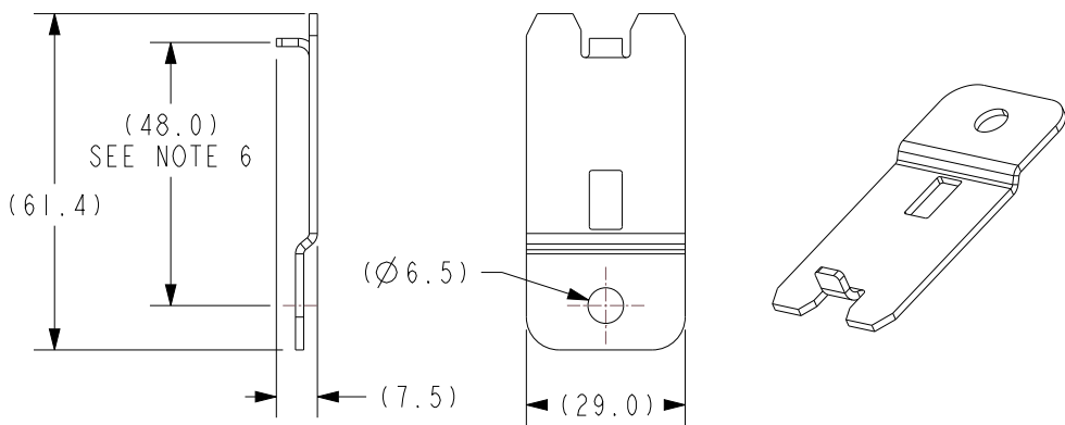
FRH-A12-MB-A2 BRACKET - PDM, FRH, FLAT WITH ANTI-ROTATION, STAINLESS 304
