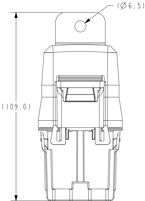
EXAMPLE CONFIGURATION WITH DIMENSIONAL INFO
