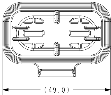
SC42-2007B-B001 HOUSING AND SEAL - PDM - FRH MAXI - 58V
