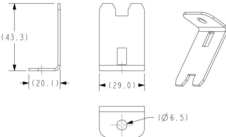
FRH-A12-MB-C1 BRACKET - PDM, FRH, 90° BENT, ZINC STEEL
