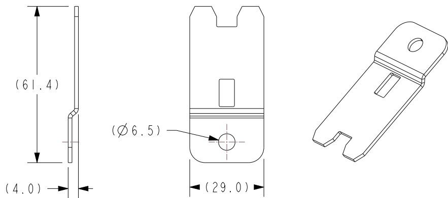
FRH-A12-MB-B1 BRACKET - PDM, FRH, FLAT WITHOUT ANTI-ROTATION, ZINC STEEL
