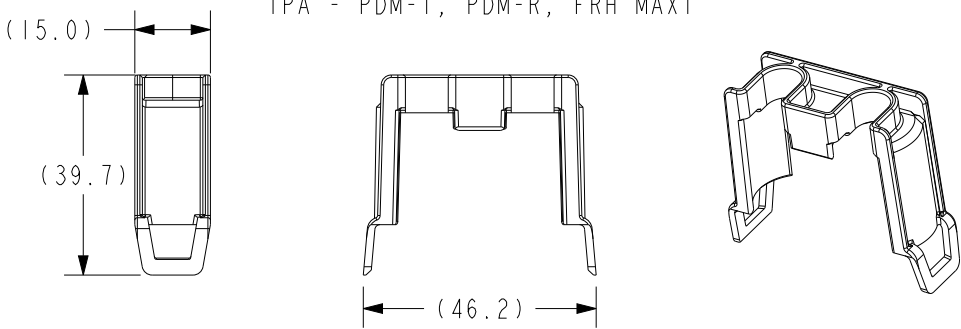
PDM-TT4 TPA - PDM-T, PDM-R, FRH MAXI
