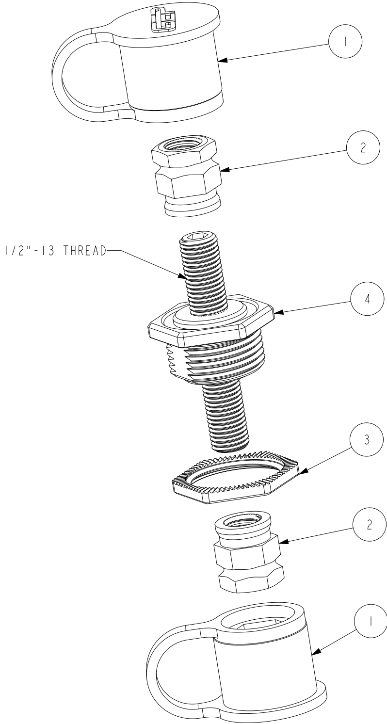
EXPLODED VIEW
