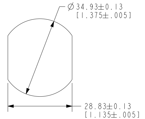
TYPICAL PANEL CUTOUT
