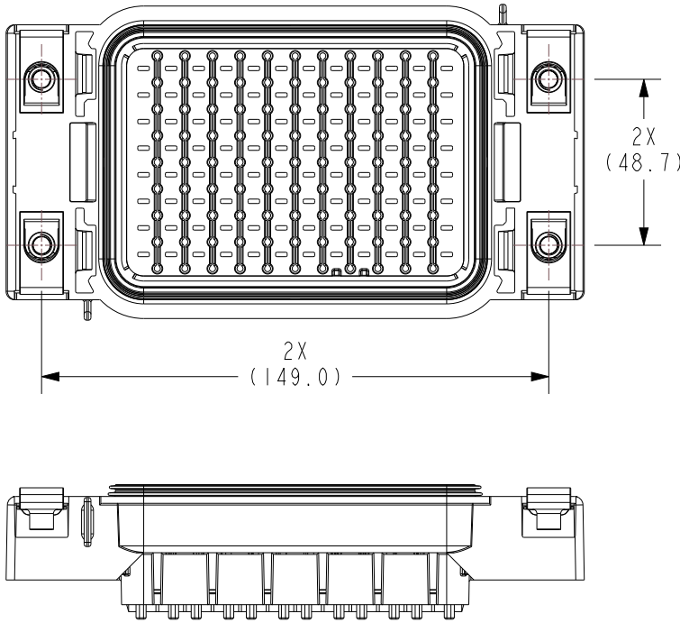
SC42-2036A-A001 HOUSING AND SEAL - PDM-U - 280 TERM - TM CLPS
