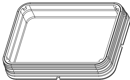
SC14-2008A-B015 COVER SEAL BLUE (ENHANCED SEALING AND UL94 V0) (INCLUDED WITH SC42-2008A-B001, SC42-2008B-B001, SC42-2036A-A001, AND SC42-2036B-A001)
