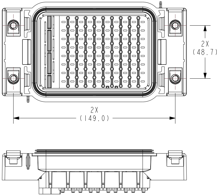
SC42-2036B-A001 HOUSING AND SEAL - PDM-U - 280 AND ATO TERM - TM CLPS
