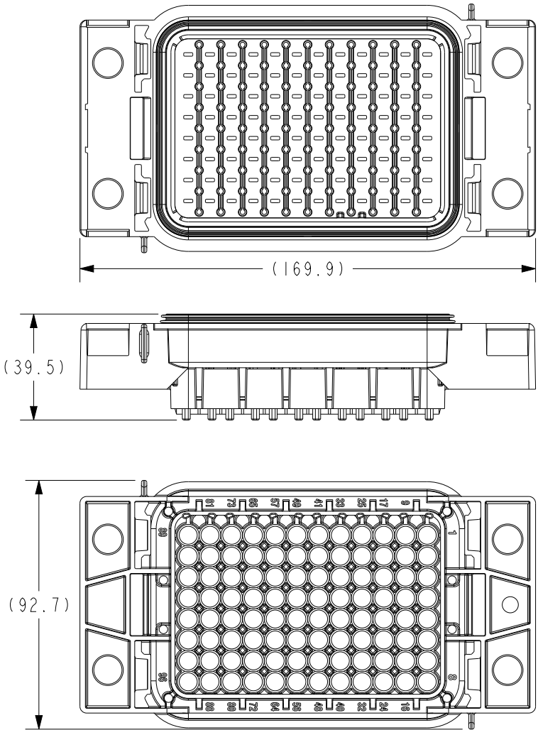
SC42-2008A-B001 HOUSING AND SEAL - PDM-U, 96 POS, 280 TERM, 10MM SEE NOTE 4
