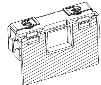
SECTION A-A EXAMPLE TAB MOUNTING
