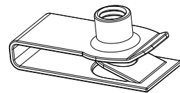
PDM-SMC (TOP) MOUNTING CLIP M6 SCALE 1:1
