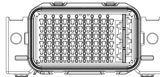
SC42-2034B-A001 HOUSING AND SEAL - PDM-S - 280 AND ATO TERM - SM CLPS
