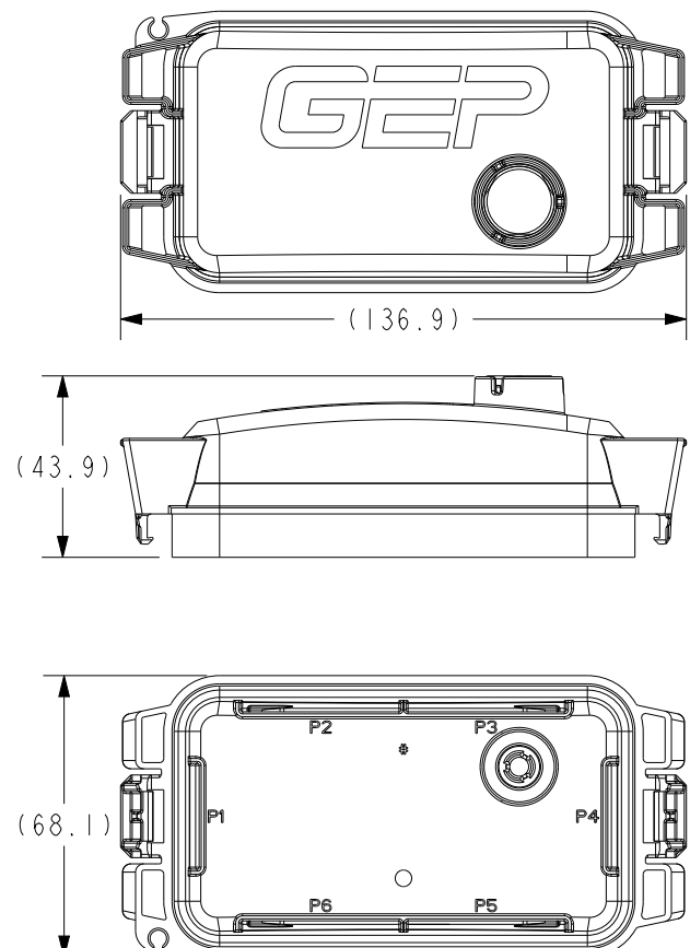
SC42-2019A-A001 COVER WITH VENT - PDM-S - GEP
