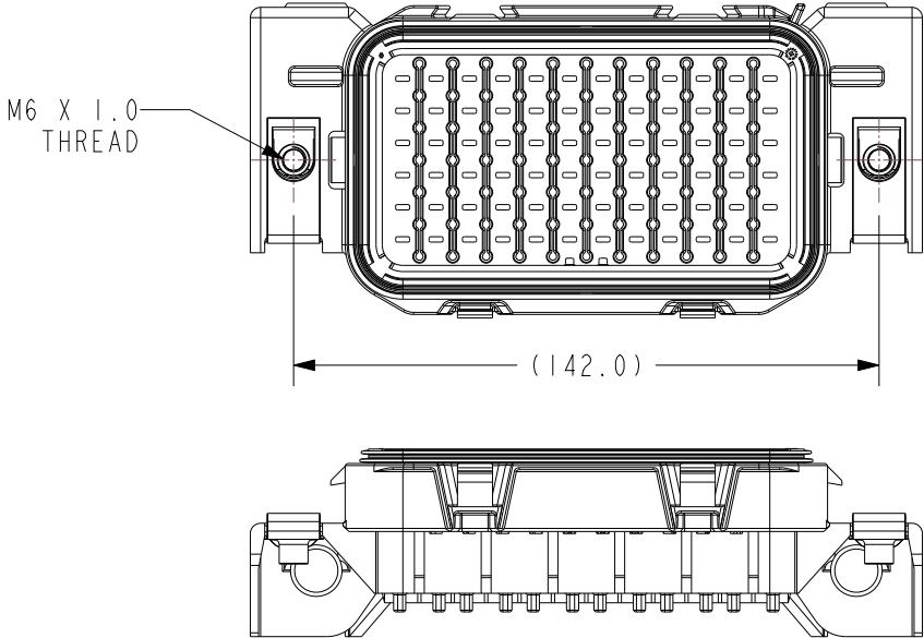
SC42-2035A-A001 HOUSING AND SEAL - PDM-S - 280 TERM - TM CLPS
