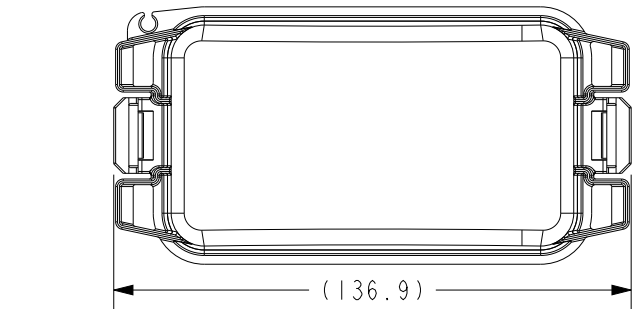
SC27-2000A-B001 COVER - PDM-S, PLAIN
