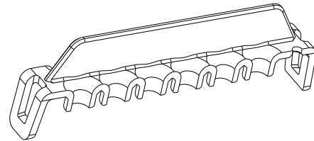
SC38-2000A-B003 TPA - PDM-S, 280 TERM (USE 6 PER ASSY FOR SC42-2005A-B001, SC42-2034A-A001, SC42-2035A-A001) (USE 5 PER ASSY FOR SC42-2005B-B001, SC42-2034B-A001, SC42-2035B-A001) SCALE 1:1
