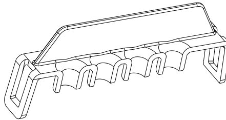
SC38-2001A-B003 TPA - PDM-S, ATO TERM (USE 1 PER ASSY FOR SC42-2005A-B001, SC42-2034B-A001, SC42-2035B-A001) SCALE 1:1
