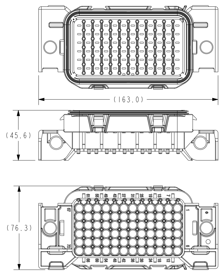
SC42-2005A-B001 HOUSING AND SEAL - PDM-S, 72 POS, 280 TERM SEE NOTE 4
