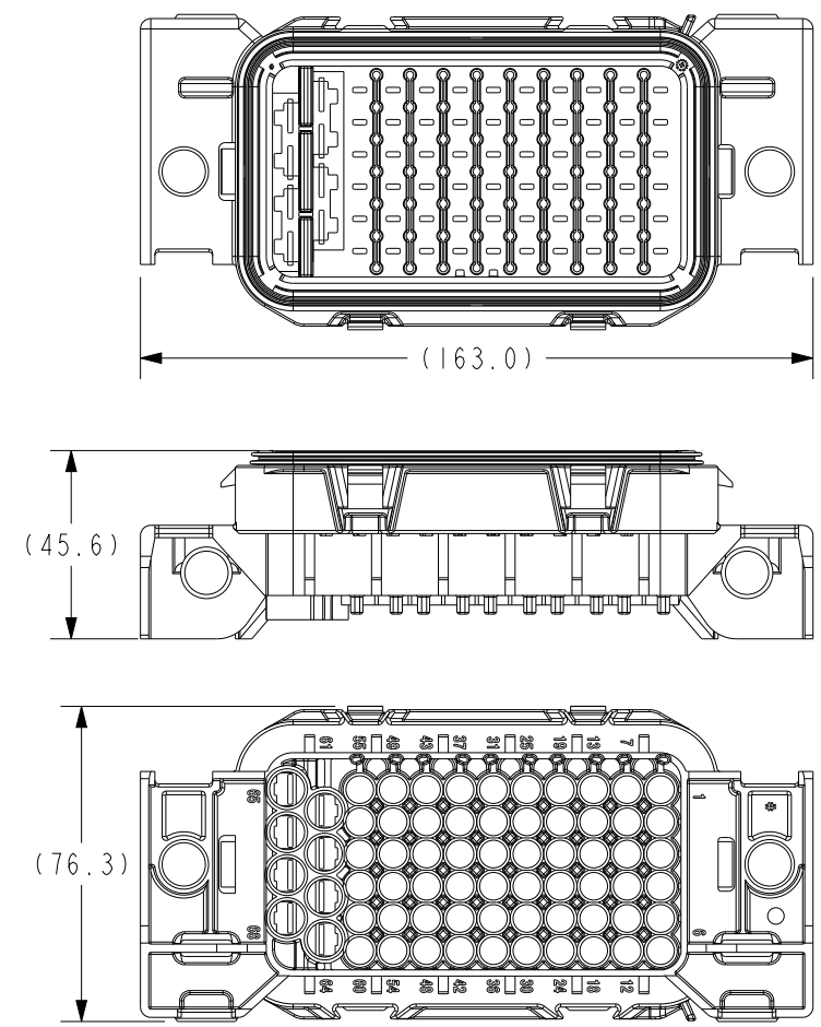
SC42-2005B-B001 HOUSING AND SEAL - PDM-S, 68 POS, 280 AND ATO TERM SEE NOTE 5
