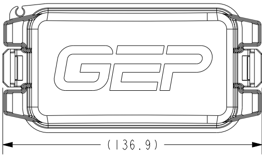
SC27-2000B-B001 COVER - PDM-S, GEP
