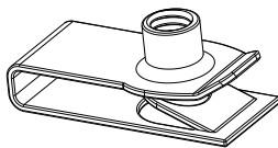
PDM-SMC (TOP) MOUNTING CLIP M6 SCALE 1:1
