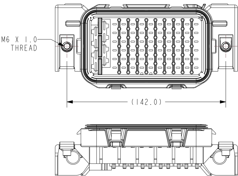
SC42-2035B-A001 HOUSING AND SEAL - PDM-S - 280 AND ATO TERM - TM CLPS
