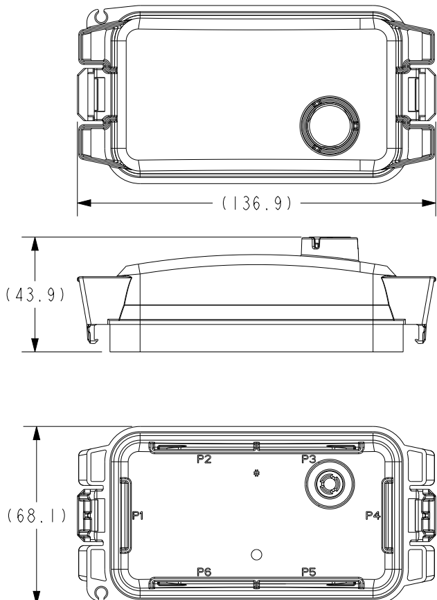
SC42-2016A-A001 COVER WITH VENT - PDM-S - PLAIN
