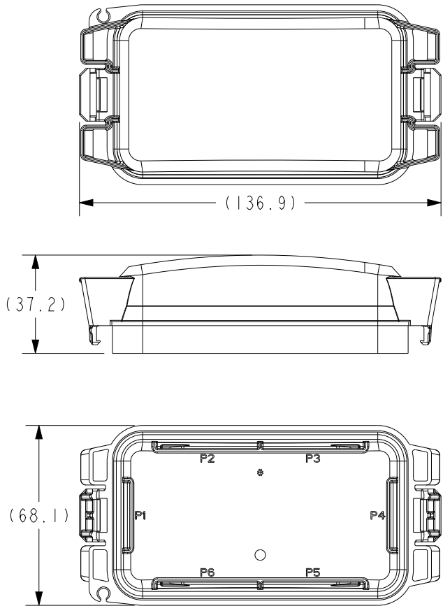
SC27-2000A-B001 COVER - PDM-S, PLAIN
