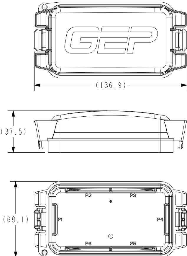
SC27-2000B-B001 COVER - PDM-S, GEP
