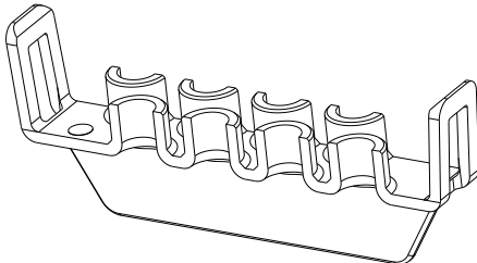
SC38-2001A-B003 TPA - PDM-S, ATO TERM (SEE TABLE T) SCALE 1:1
