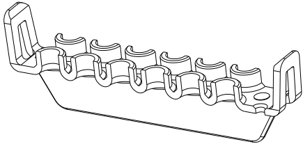
SC38-2000A-B003 TPA - PDM-S, 280 TERM (SEE TABLE T) SCALE 1:1
