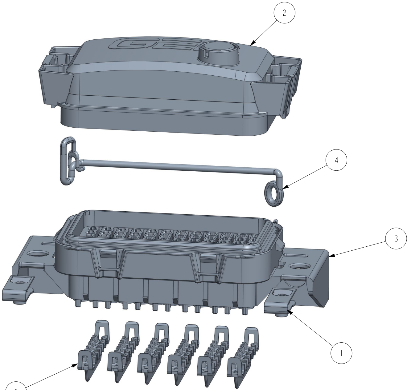
EXAMPLE CONFIGURATION EXPLODE VIEW
