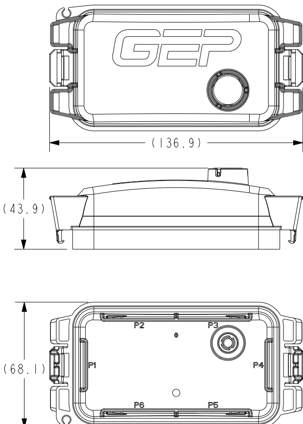
SC42-2019A-A001 COVER WITH VENT - PDM-S - GEP
