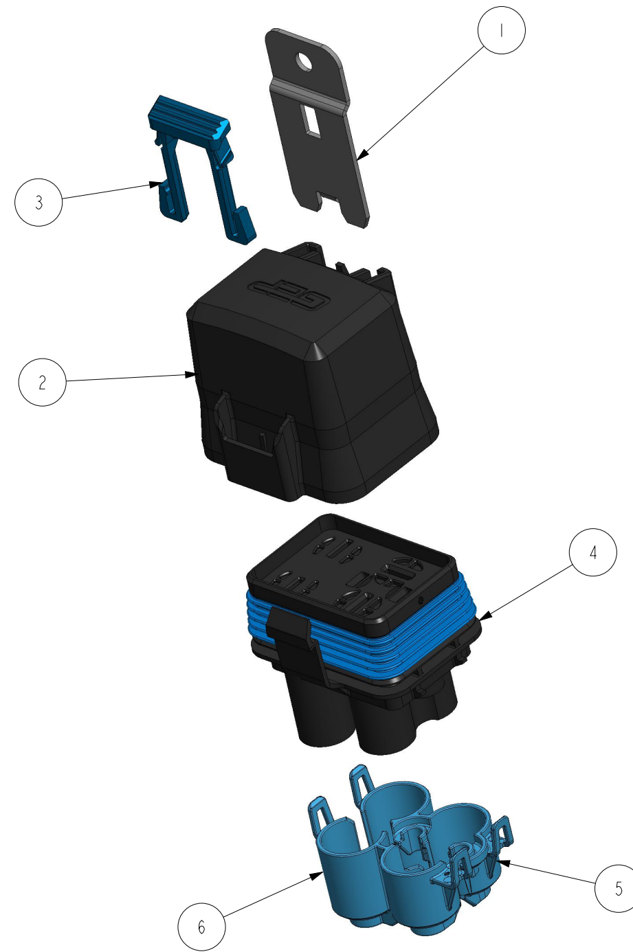
EXAMPLE CONFIGURATION EXPLODE VIEW
