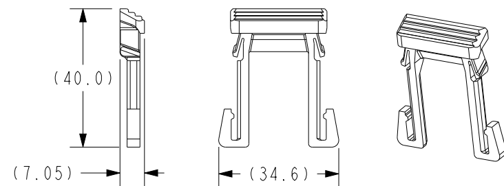
FRH-A-CPA CPA - PDM, FRH
