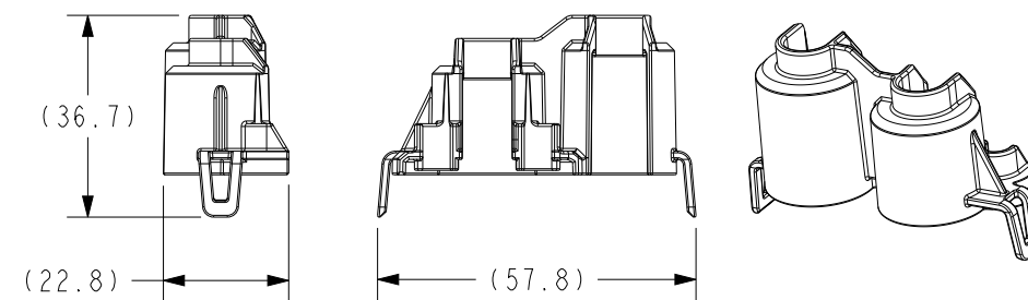
SC38-2015A-B003 TPA - FRH - MAXI ISO RELAY AND MAXI FUSE - A SIDE
