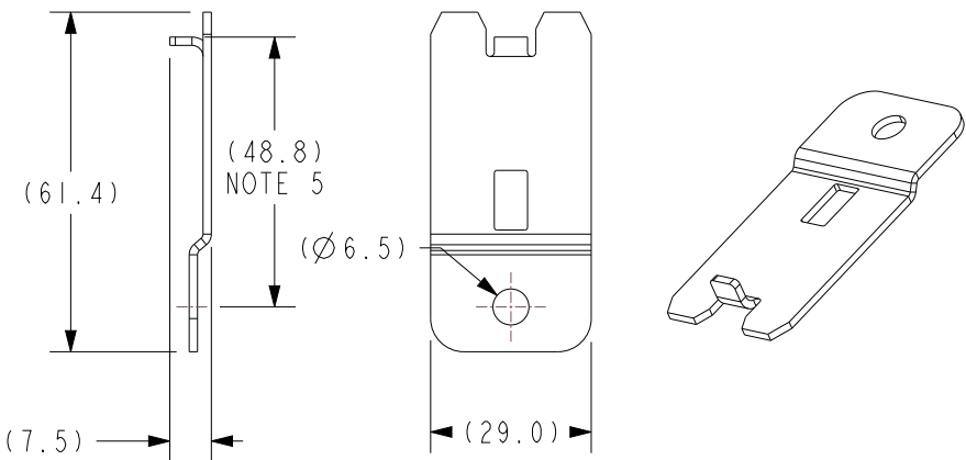
FRH-A12-MB-A1 BRACKET - PDM,FRH,FLAT WITH ANTI-ROTATION, ZINC STEEL
