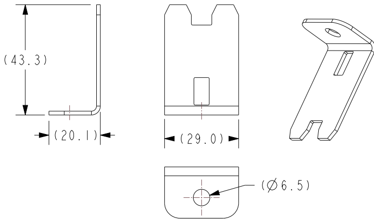
FRH-A12-MB-C1 BRACKET - PDM, FRH, 90° BENT, ZINC STEEL
