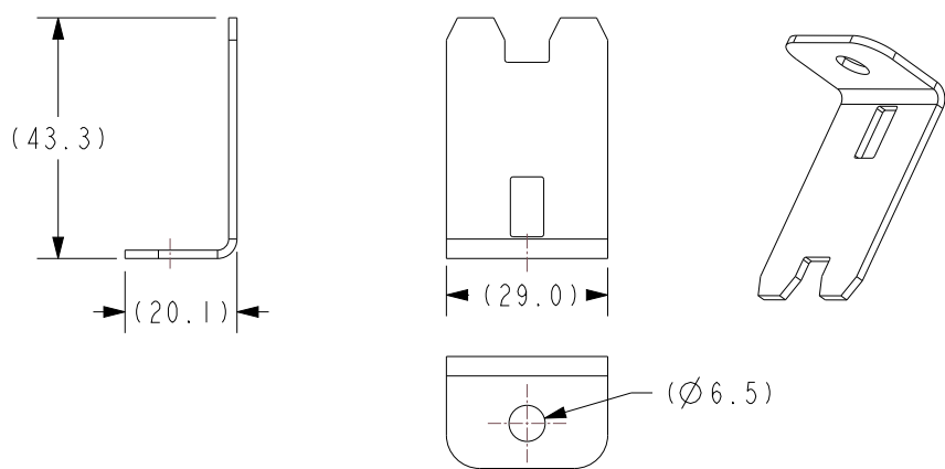
FRH-A12-MB-C2 BRACKET - PDM, FRH, 90° BENT, STAINLESS 304
