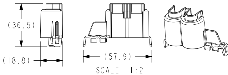
SC38-2013B-B003 TPA - PDM, FRH, MAXI AND MINI, B
