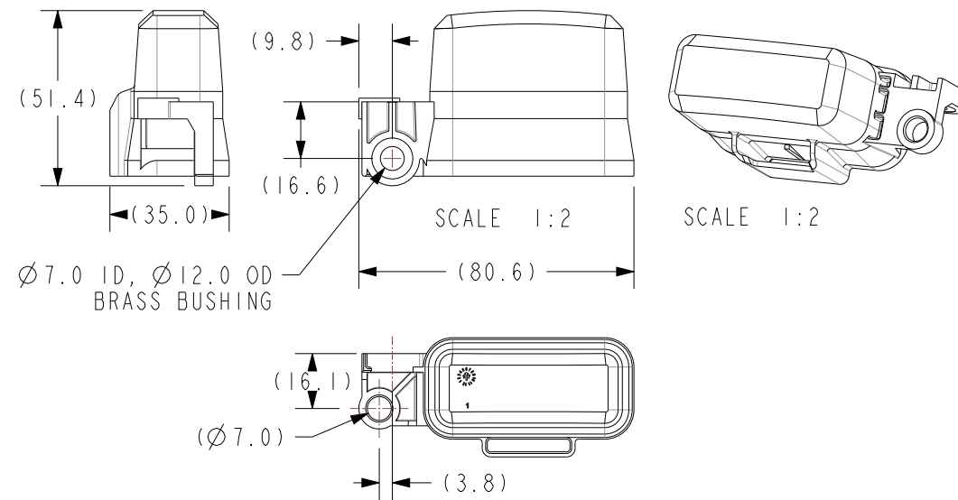
FRH-A12-CB-1 COVER - PDM, FRH 12 POS, SINGLE SIDE MOUNT, PLAIN
