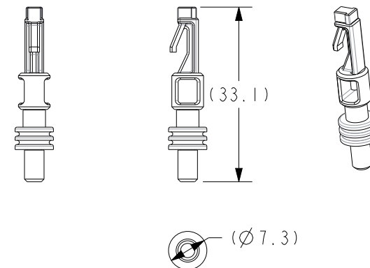
SC55-2000A-A001 PLUG AND SEAL - PDM CAVITY PLUG - METRIPACK 280
