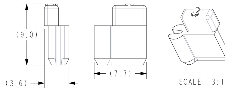
PDM-TK DIODE KEY
