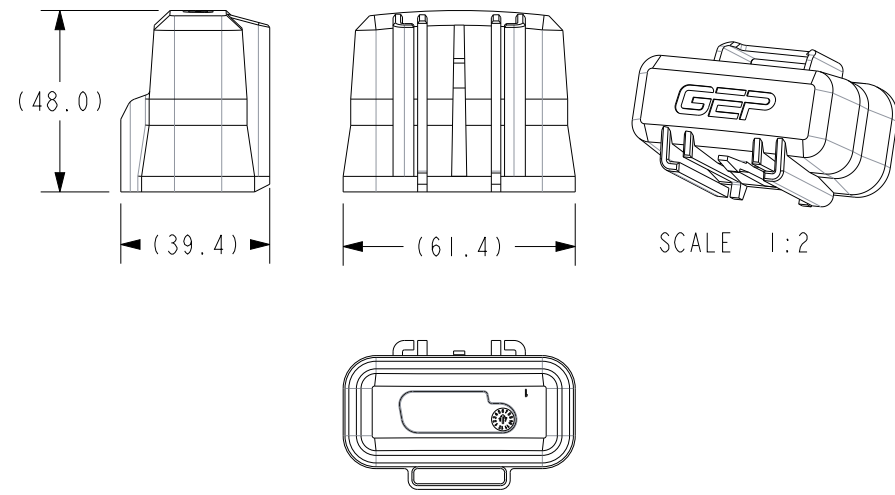
SC42-2027A-A001 COVER WITH VENT - FRH - A12
