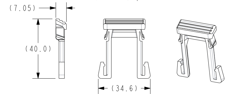
FRH-A-CPA CPA - PDM, FRH
