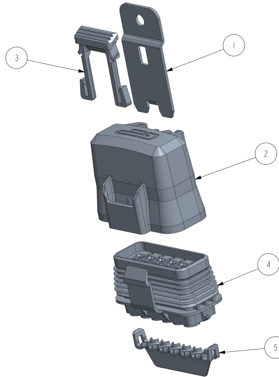
EXAMPLE CONFIGURATION EXPLODE VIEW
