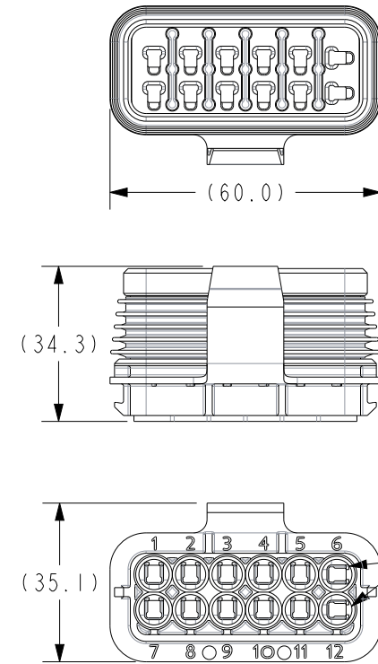
SC42-2018A-A001 HOUSING AND SEAL - PDM FRH 12 POS - ROTATED FUSE (FOR TERMINALS AND SEALS SEE TABLE A)
